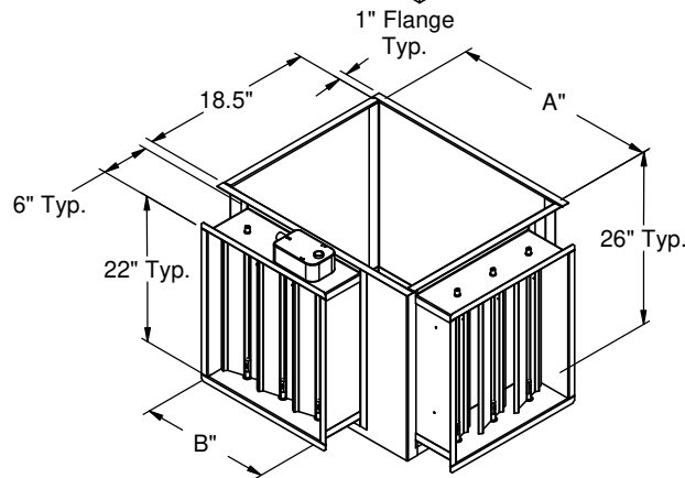
Damper Example Shown P/N: MB-AV*-**-FA
