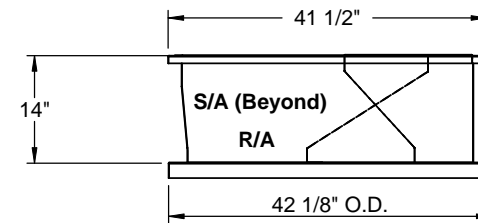
RIGHT VIEW
