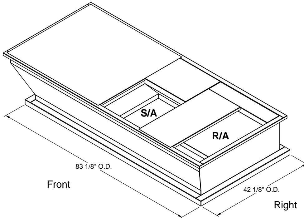
ISOMETRIC VIEW
