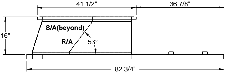
RIGHT VIEW
