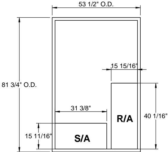
EXISTING CURB
