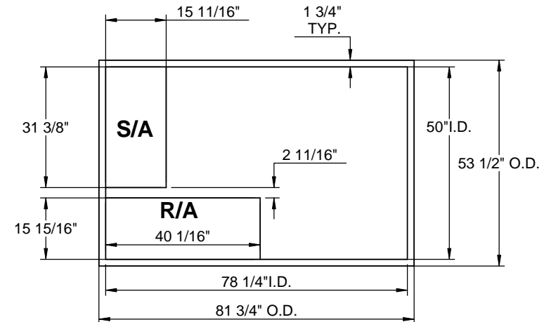
EXISTING CURB
