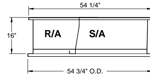
RIGHT VIEW
