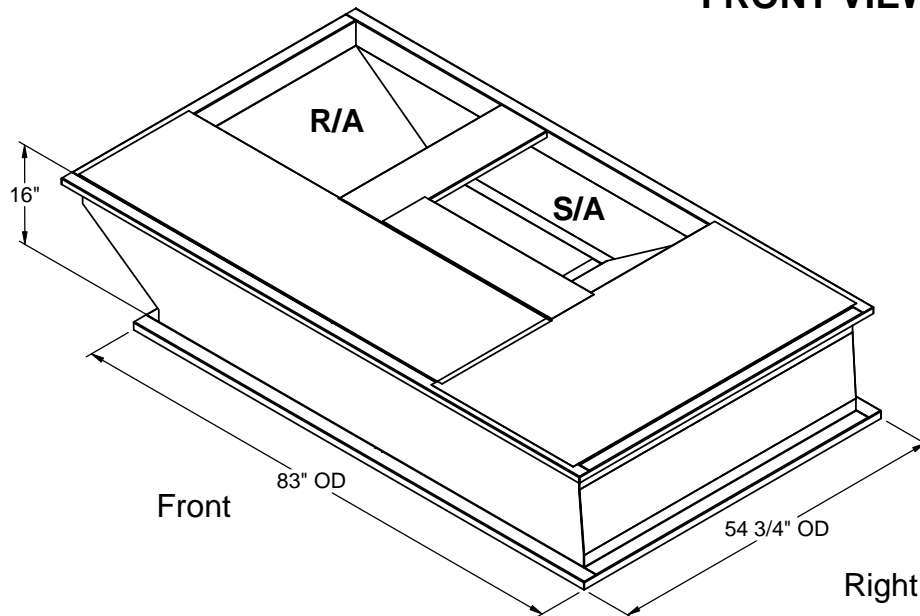
ISOMETRIC VIEW
