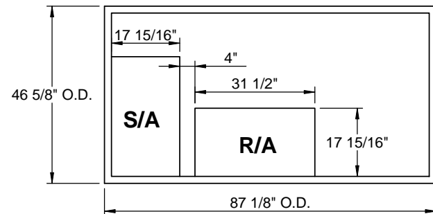
EXISTING CURB
