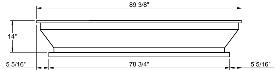
RIGHT VIEW
