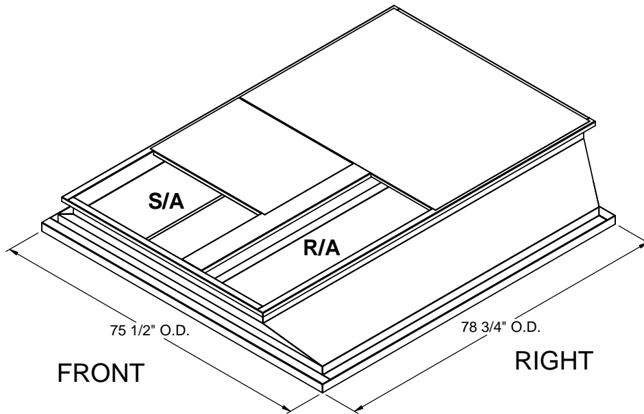
ISOMETRIC VIEW
