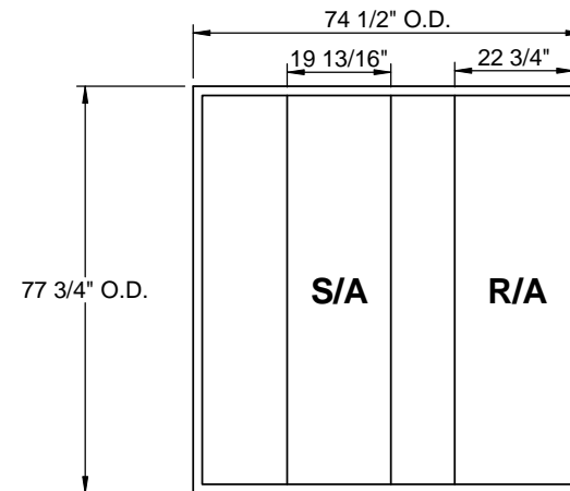
EXISTING CURB
