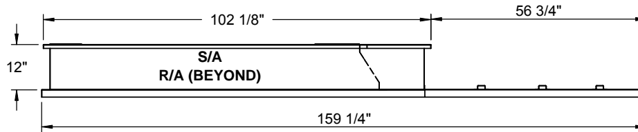
FRONT VIEW
