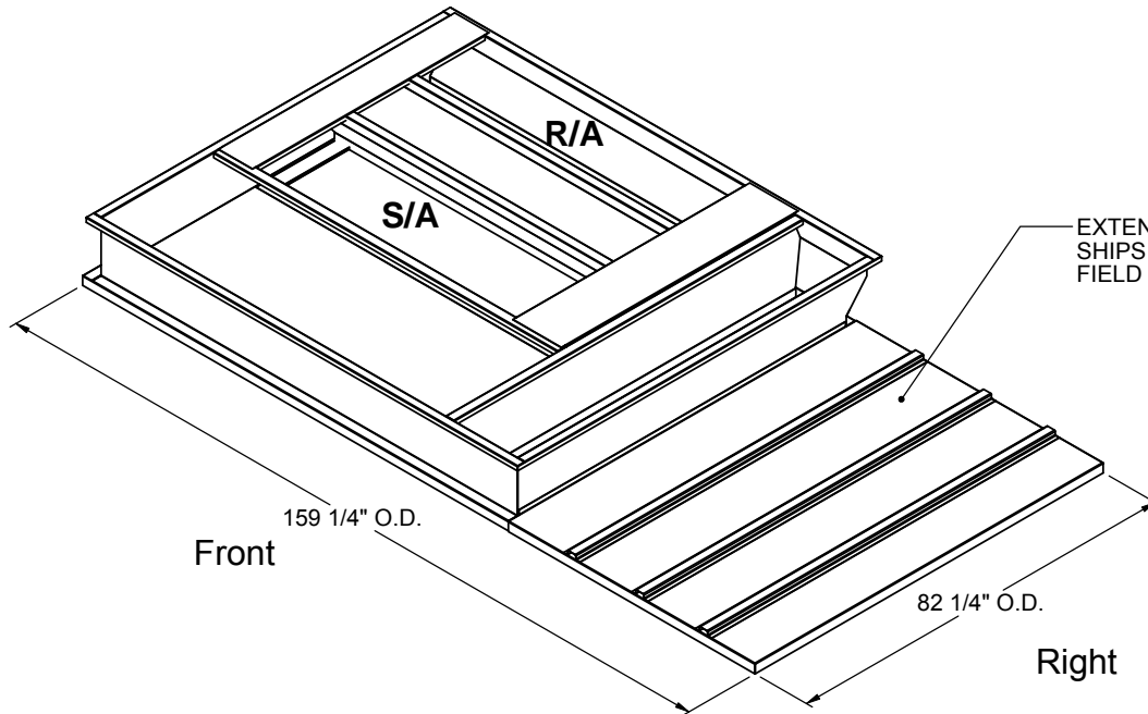
ISOMETRIC VIEW
