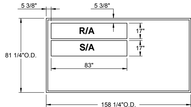
EXISTING CURB
