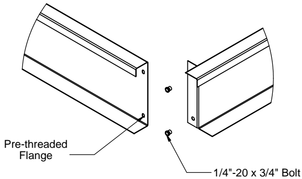
CORNER DETAIL
