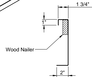
CROSS SECTION DETAIL
