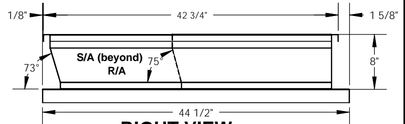
RIGHT VIEW
