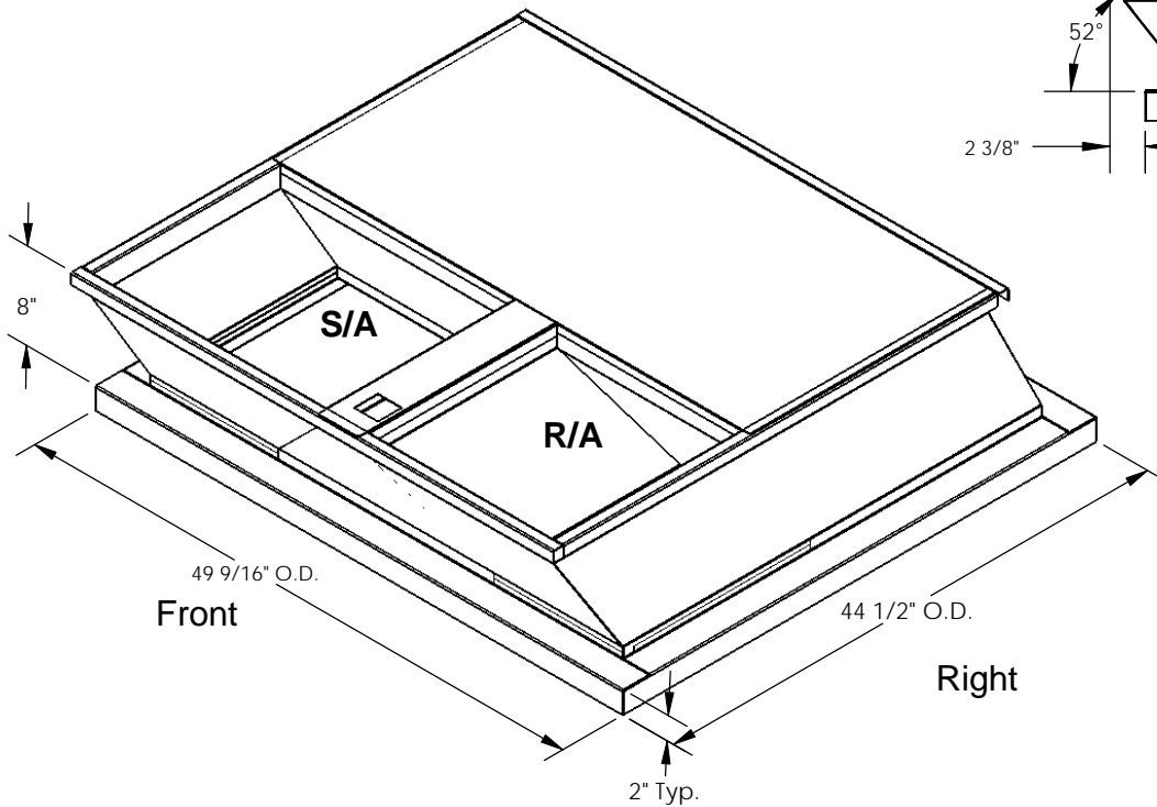
ISOMETRIC VIEW
