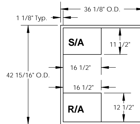
EXISTING CURB
