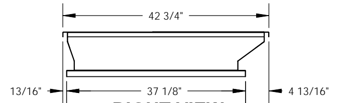
RIGHT VIEW
