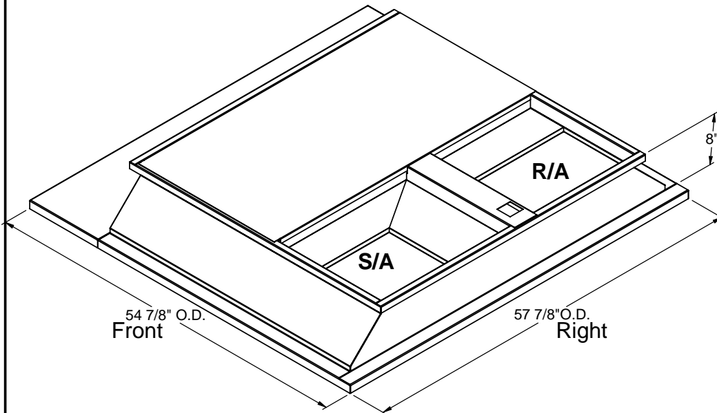
ISOMETRIC VIEW
