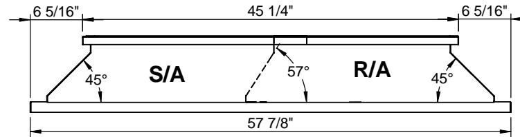
RIGHT VIEW
