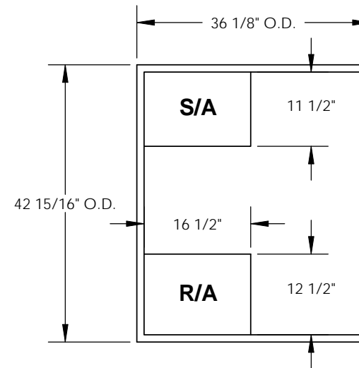
EXISTING CURB
