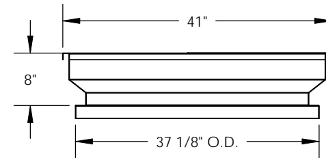
RIGHT VIEW
