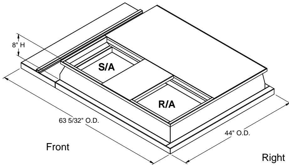
ISOMETRIC VIEW
