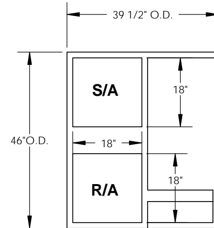
EXISTING CURB
