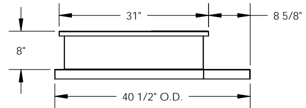
RIGHT VIEW
