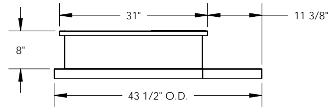
RIGHT VIEW
