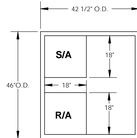
EXISTING CURB
