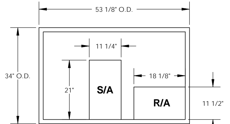
EXISTING CURB
