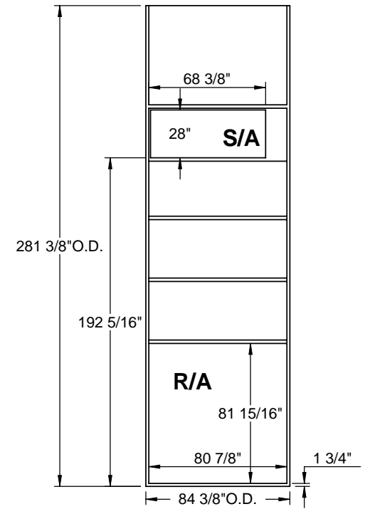
EXISTING CURB
