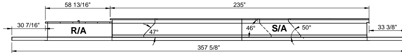
RIGHT VIEW
