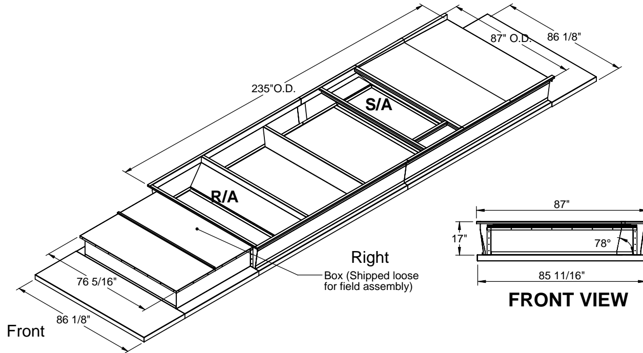
ISOMETRIC VIEW
