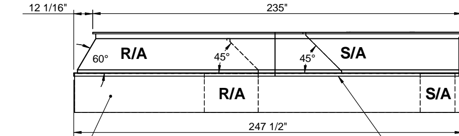
RIGHT VIEW
