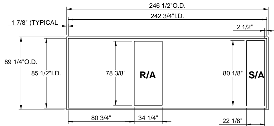
EXISTING CURB
