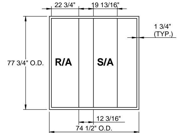
EXISTING CURB
