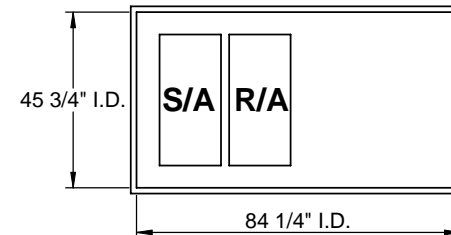
EXISTING CURB
