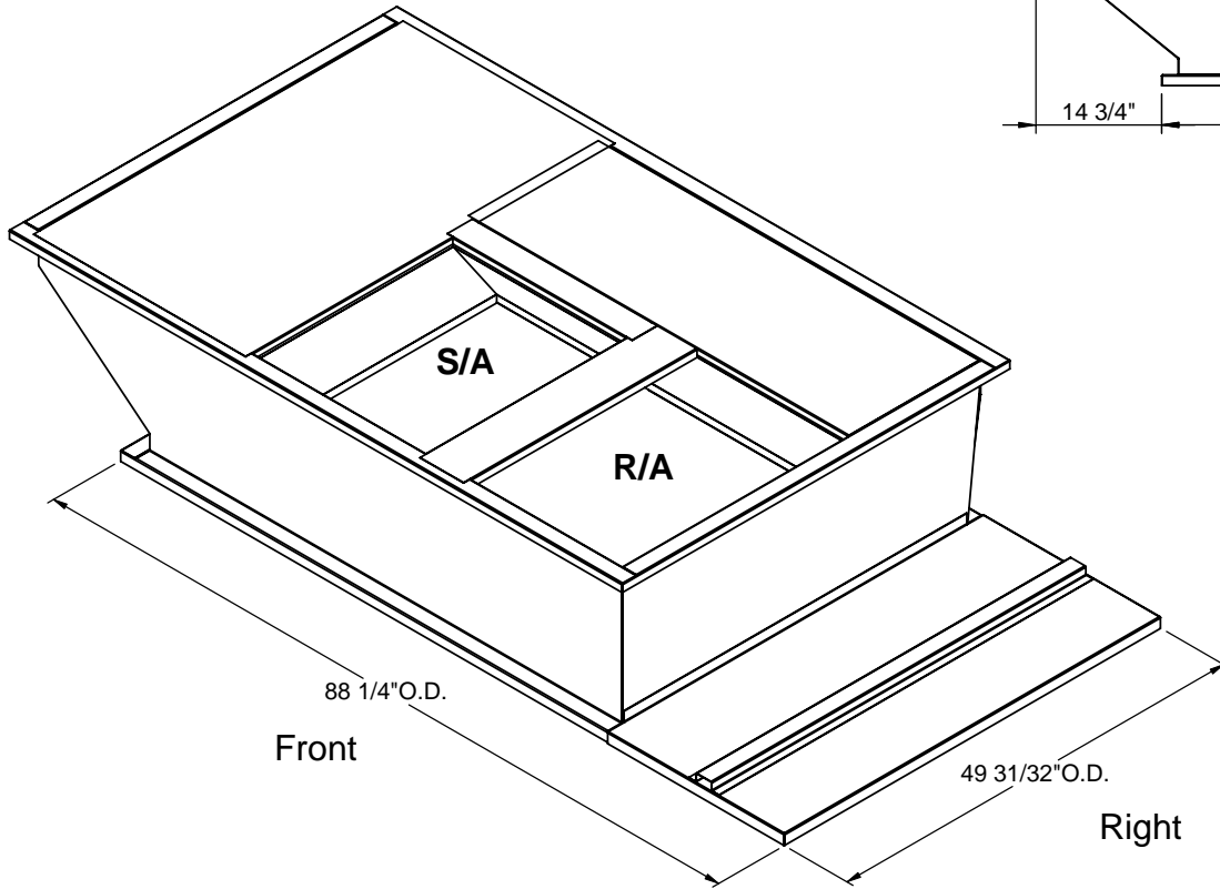
ISOMETRIC VIEW
