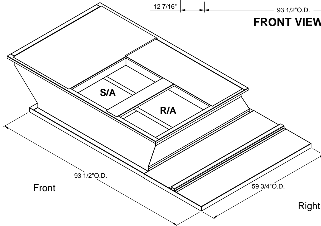
ISOMETRIC VIEW
