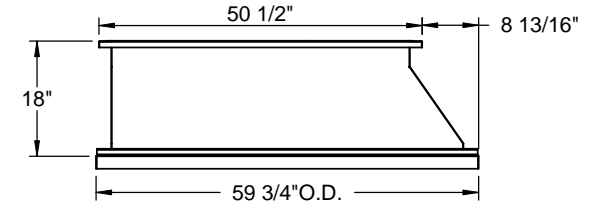
RIGHT VIEW
