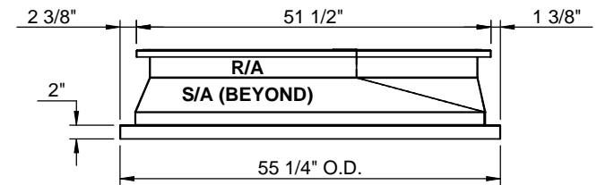
RIGHT VIEW
