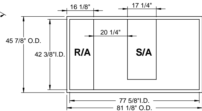
EXISTING CURB
