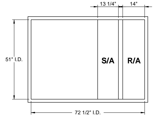
EXISTING CURB
