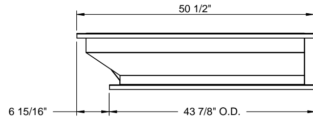
RIGHT VIEW
