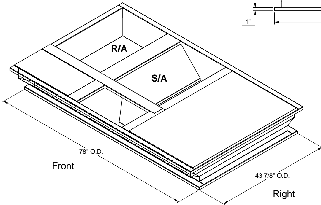
ISOMETRIC VIEW
