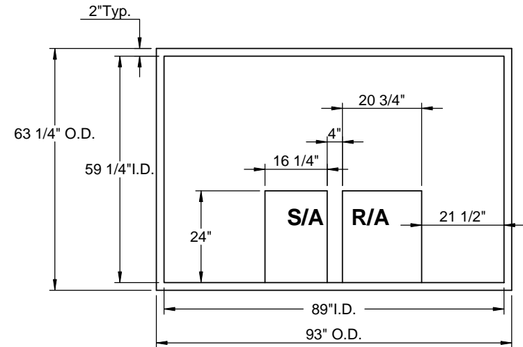
EXISTING CURB
