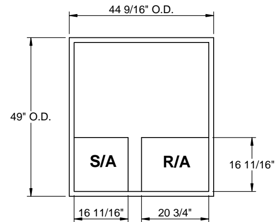
EXISTING CURB
