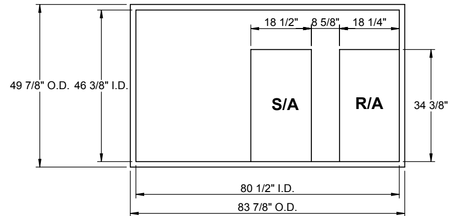
EXISTING CURB
