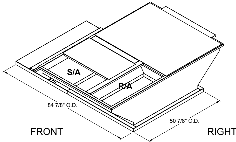
ISOMETRIC VIEW
