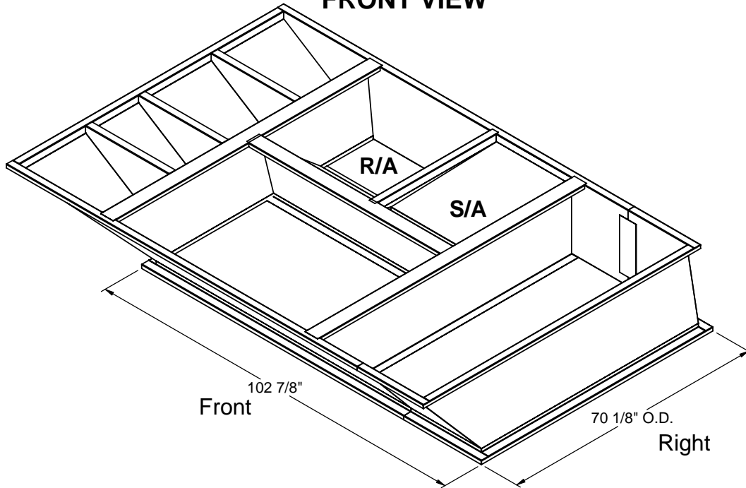
ISOMETRIC VIEW
