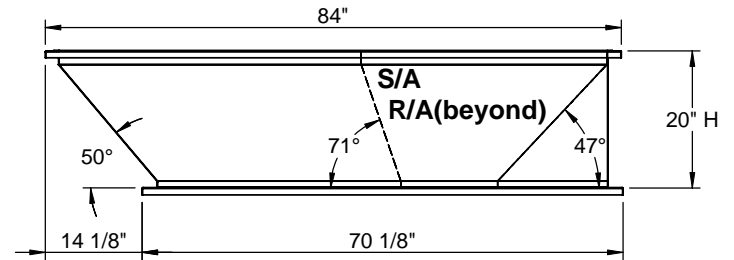
RIGHT VIEW
