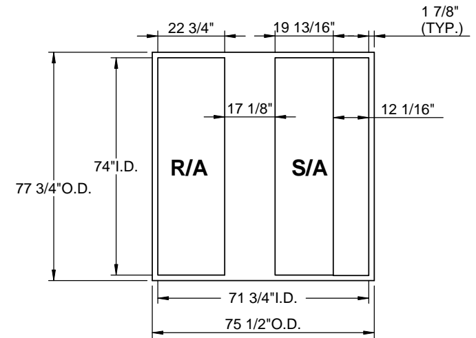
EXISTING CURB
