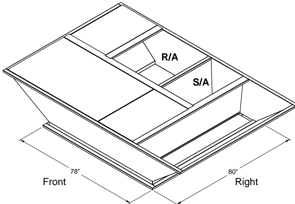
ISOMETRIC VIEW
