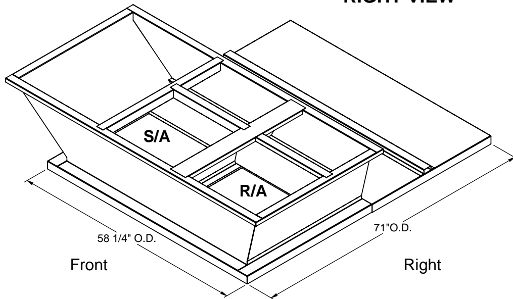
ISOMETRIC VIEW
