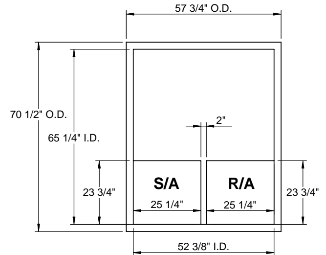
EXISTING CURB
