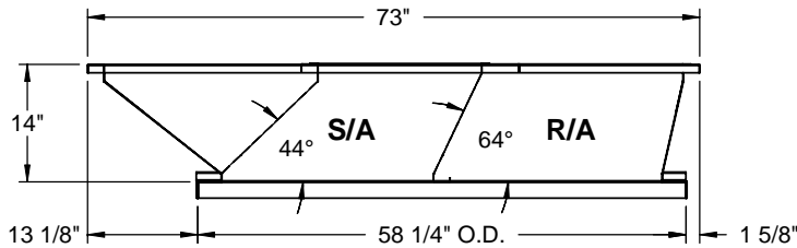
RIGHT VIEW
