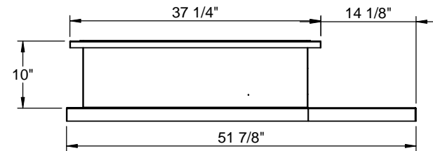
RIGHT VIEW
