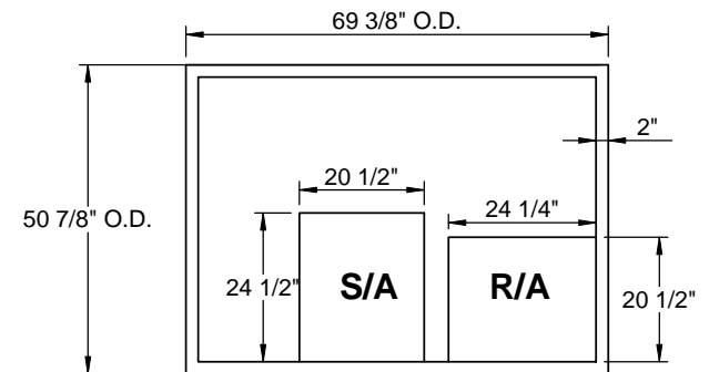
EXISTING CURB
