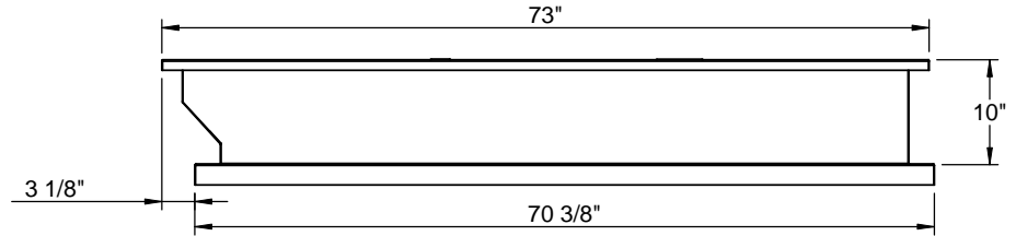
FRONT VIEW
