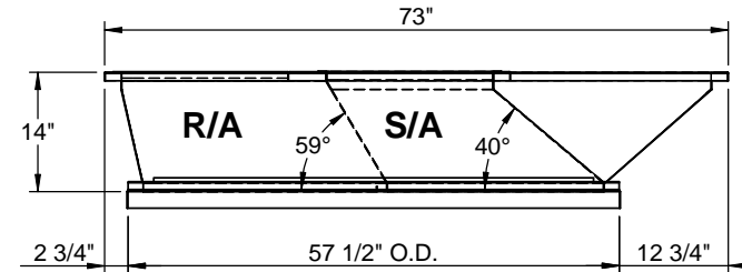
RIGHT VIEW
