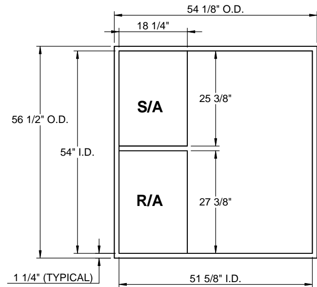
EXISTING CURB
