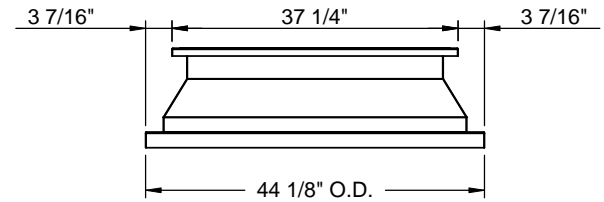
RIGHT VIEW
