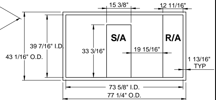
EXISTING CURB
