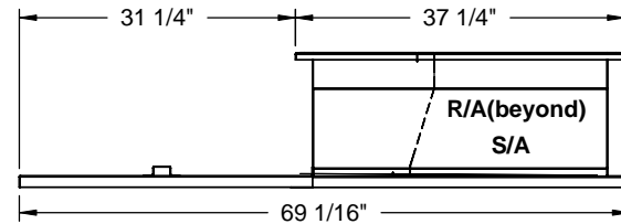
RIGHT VIEW
