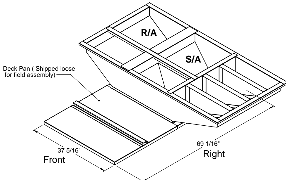
ISOMETRIC VIEW
