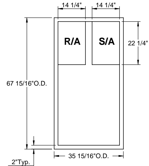
EXISTING CURB
