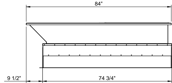
RIGHT VIEW
