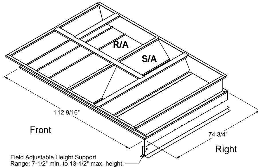
ISOMETRIC VIEW
