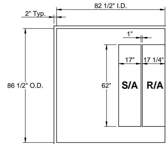
EXISTING CURB
