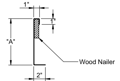
SIDE DETAIL
