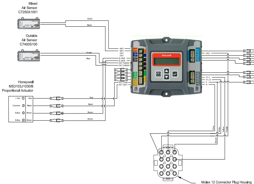
ILL. 6 Control Wiring Diagram
