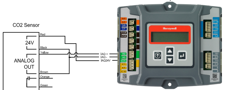
ILL. 7 Jade controller application
