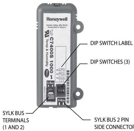
ILL. 5 Sylk Bus sensor DIP switches
