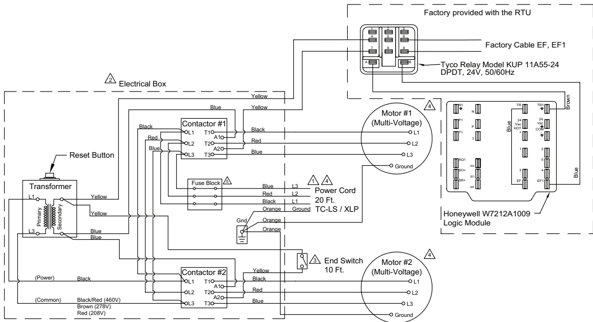
ILL. 3 - Constant Volume Power Exhaust Wiring
