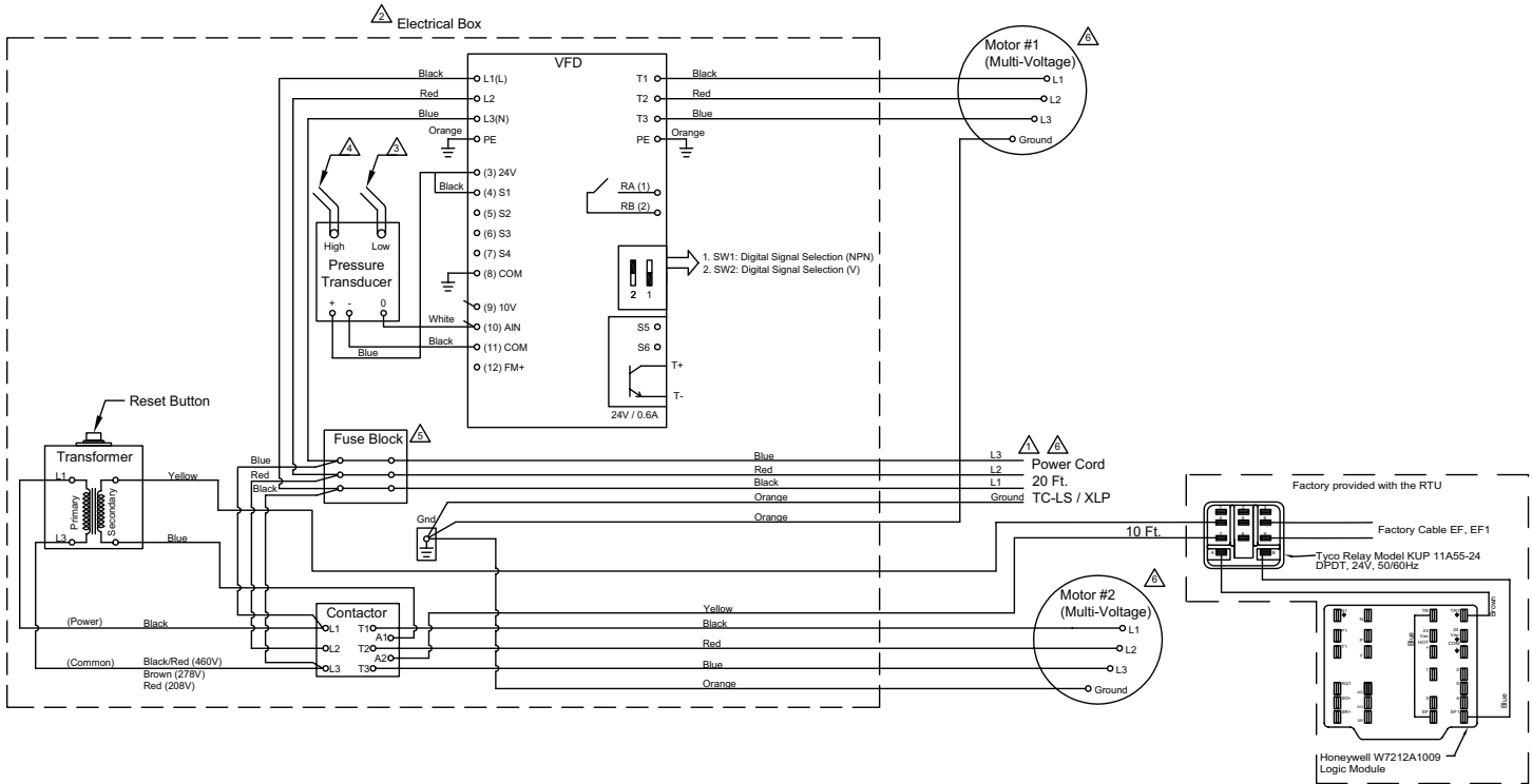
ILL. 4 - Modulating Power Exhaust Option Wiring
