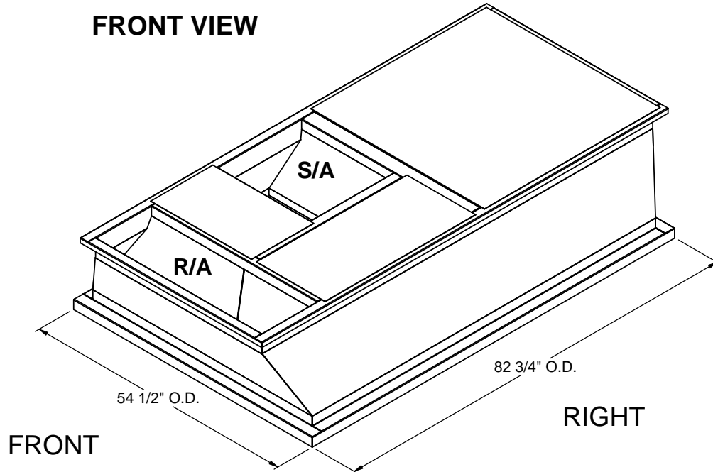
ISOMETRIC VIEW
