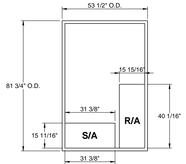
EXISTING CURB
