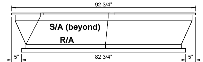
RIGHT VIEW
