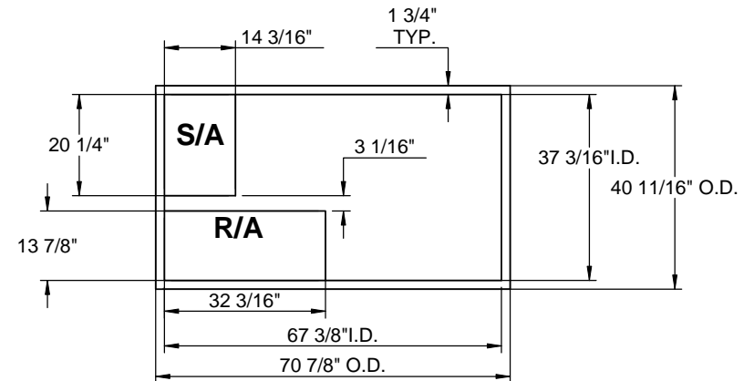
EXISTING CURB
