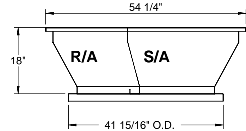
RIGHT VIEW
