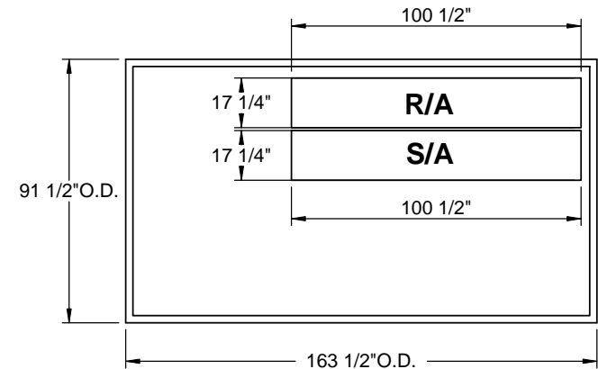
EXISTING CURB
