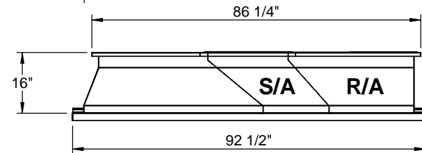
RIGHT VIEW
