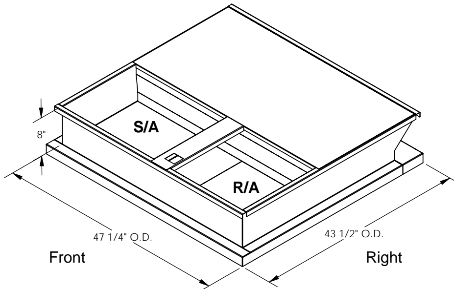
ISOMETRIC VIEW
