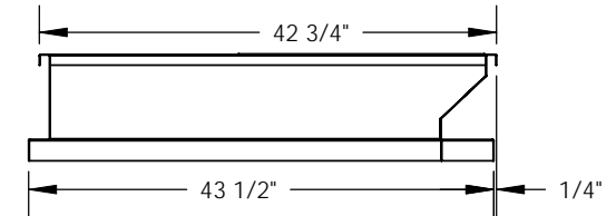
RIGHT VIEW
