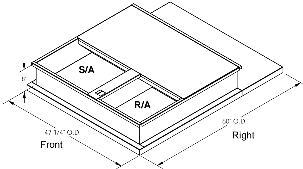
ISOMETRIC VIEW
