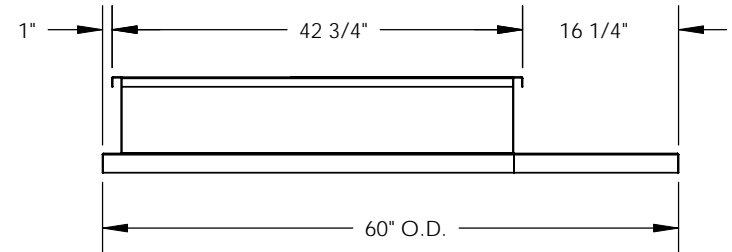
RIGHT VIEW
