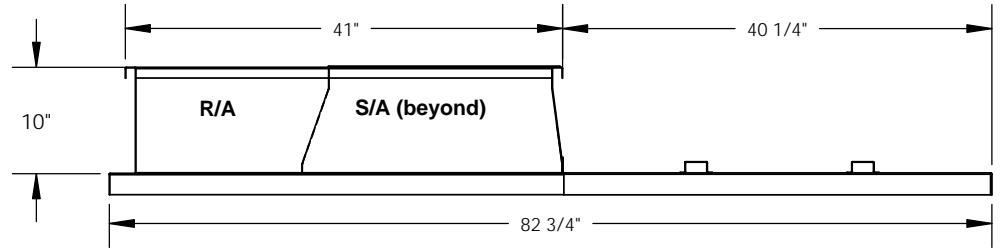
RIGHT VIEW
