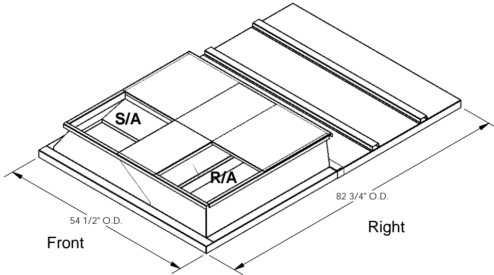
ISOMETRIC VIEW
