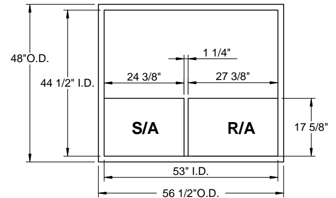
EXISTING CURB
