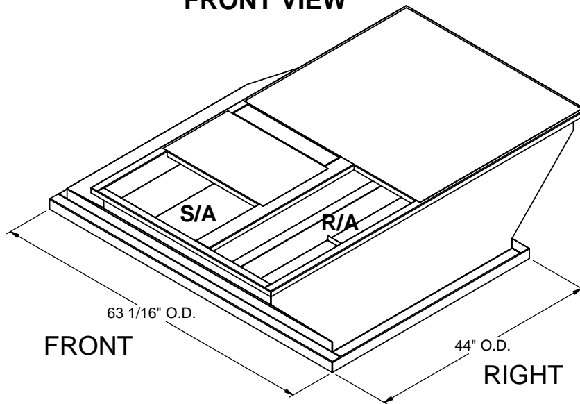
ISOMETRIC VIEW
