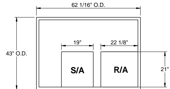
EXISTING CURB
