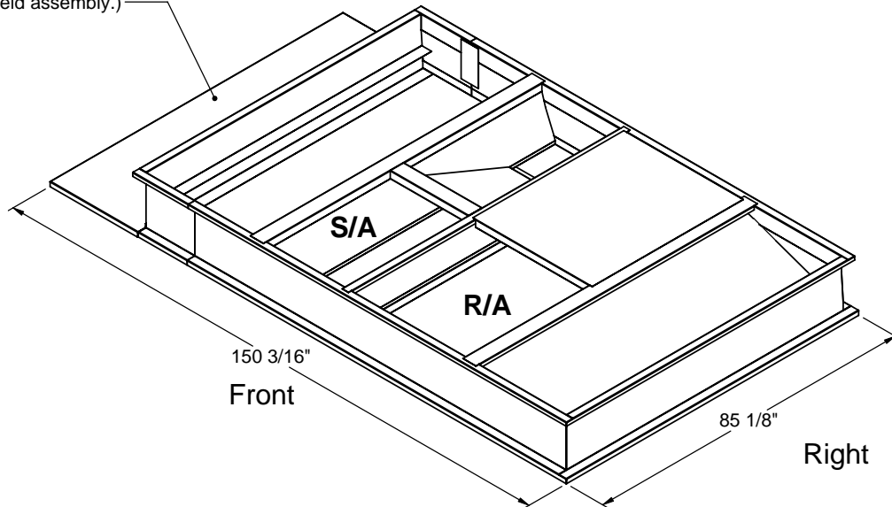
ISOMETRIC VIEW
