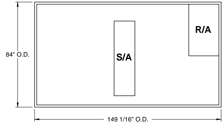
EXISTING CURB
